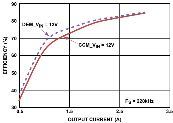
FIGURE 6. EFFICIENCY vs LOAD CURRENT AT 12V INPUT
