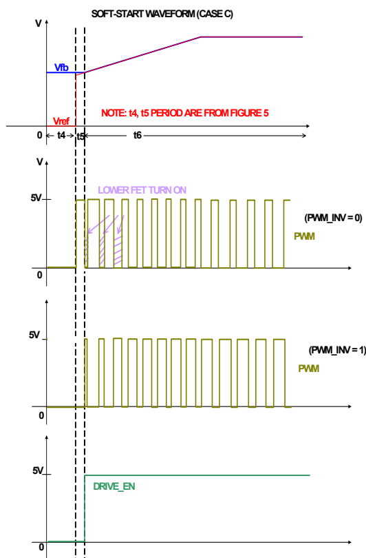
FIGURE 17. SOFT-START WAVEFORM (CASE C, LIGHT LOAD)
