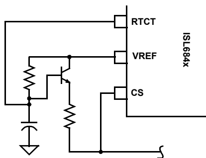
FIGURE 7. SLOPE COMPENSATION
