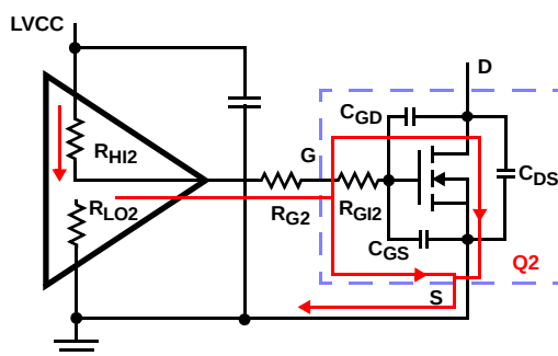
FIGURE 5. TYPICAL LOWER-GATE DRIVE TURN-ON PATH
