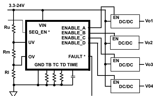
FIGURE 1. ISL870XA IMPLEMENTATION
