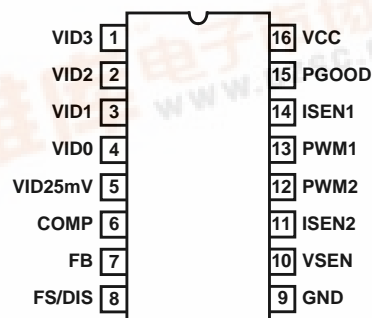
ISL6553 (SOIC) TOP VIEW
