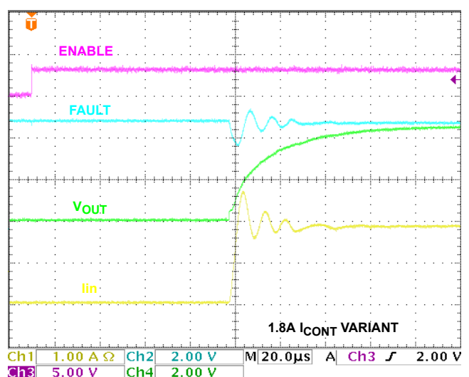
FIGURE 24. V IN = 5V TURN-ON INTO 2.7Ω
