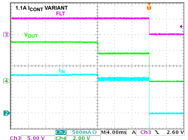
FIGURE 22. I LIM WAVEFORM
