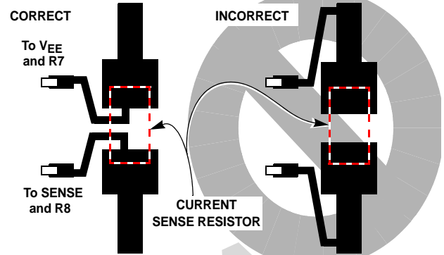
FIGURE 30. SENSE RESISTOR LAYOUT GUIDELINES
