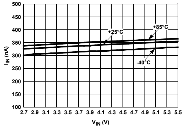
FIGURE 44. I_{IN} vs V_{IN} OVER-TEMPERATURE
