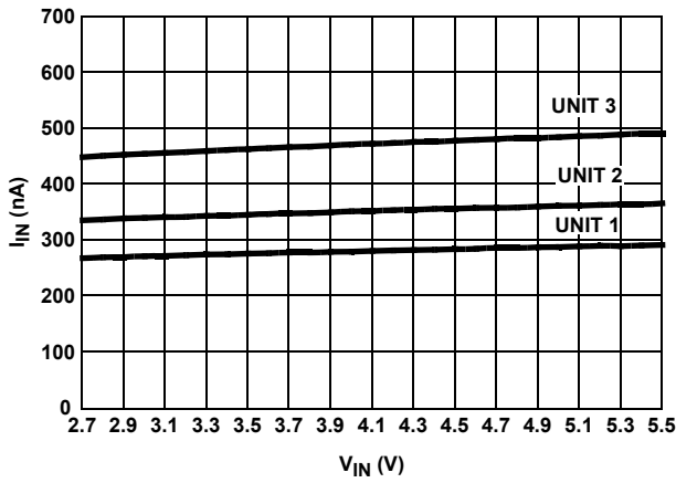
FIGURE 15. I_{IN} vs V_{IN} , 3 UNITS
