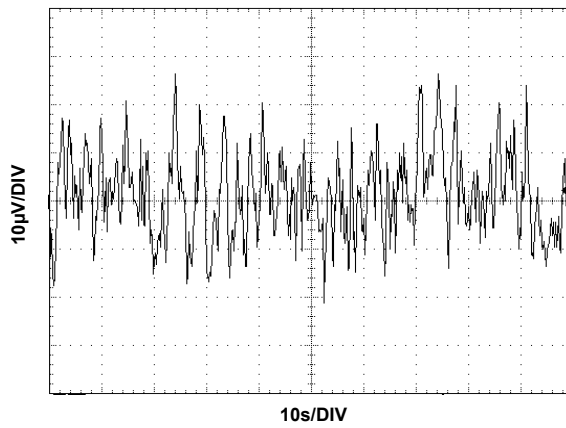
FIGURE 28. V_{OUT} NOISE
