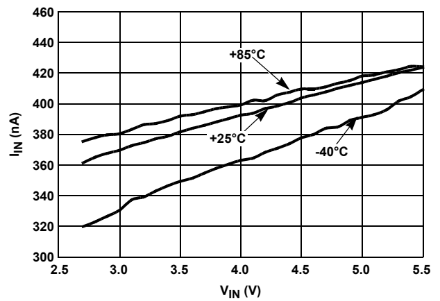
FIGURE 71. I_{IN} vs V_{IN} OVER-TEMPERATURE
