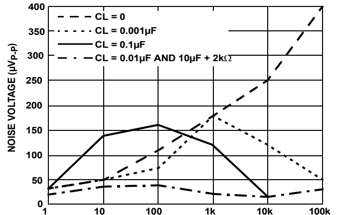
FIGURE 118. NOISE REDUCTION
