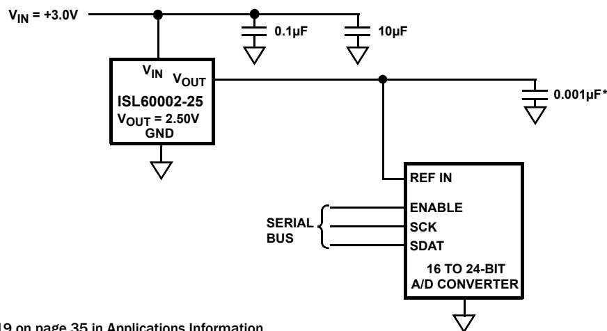
FIGURE 1. TYPICAL APPLICATION
