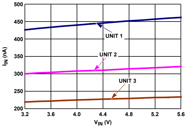
FIGURE 84. I_{IN} vs V_{IN} , 3 UNITS
