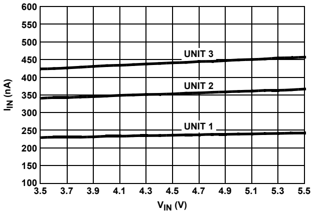
FIGURE 99. I_{IN} vs V_{IN} , 3 UNITS
