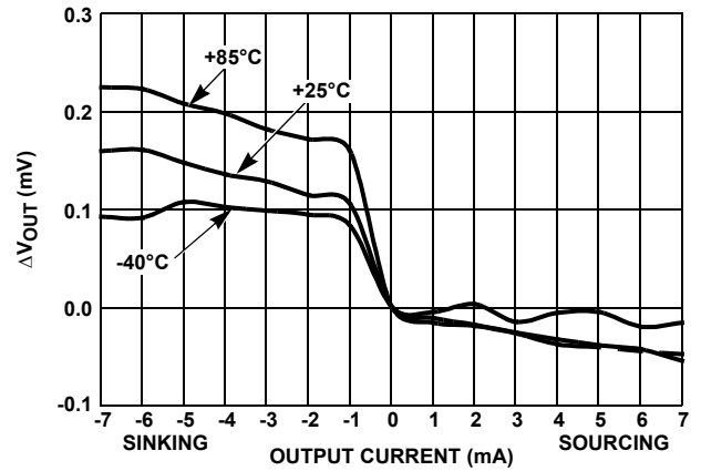
FIGURE 37. LOAD REGULATION
