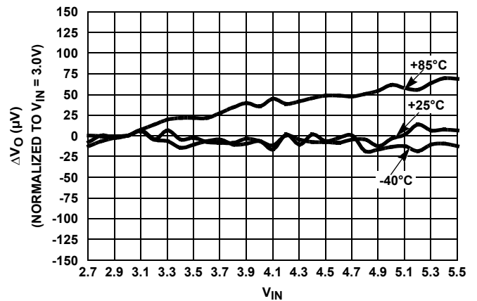
FIGURE 19. LINE REGULATION OVER-TEMPERATURE
