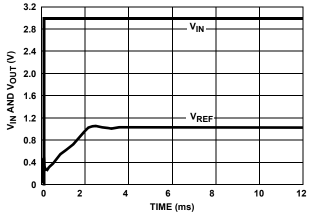
FIGURE 13. TURN-ON TIME (+25°C)
