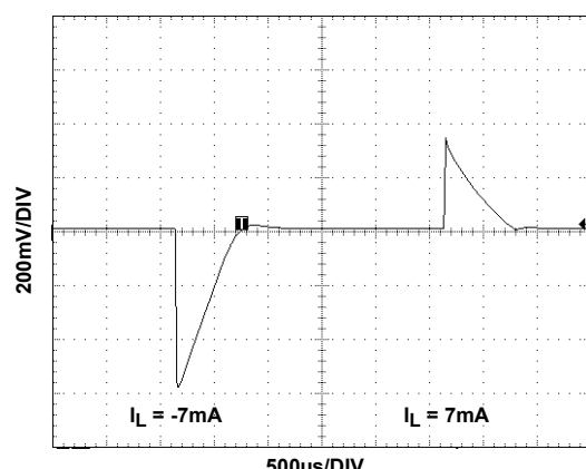
FIGURE 80. LOAD TRANSIENT RESPONSE
