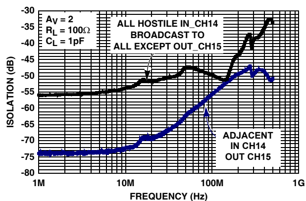
FIGURE 12. CROSSTALK - A_V = 2
