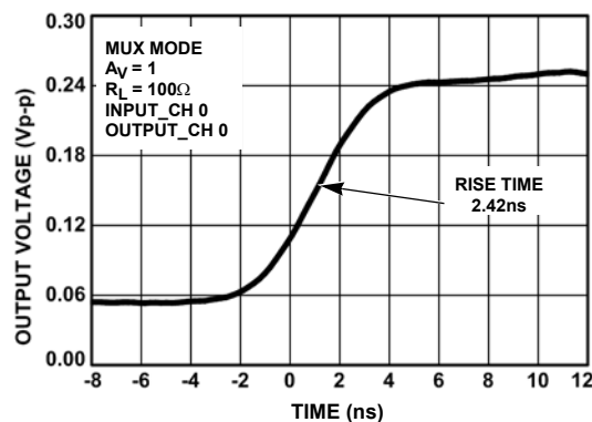
FIGURE 17. RISE TIME - A_V = 1
