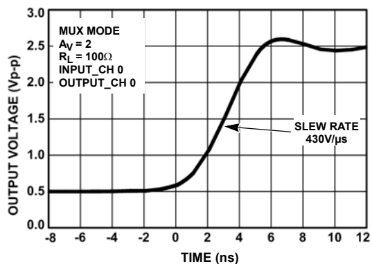
FIGURE 23. RISING SLEW RATE - A_V = 2
