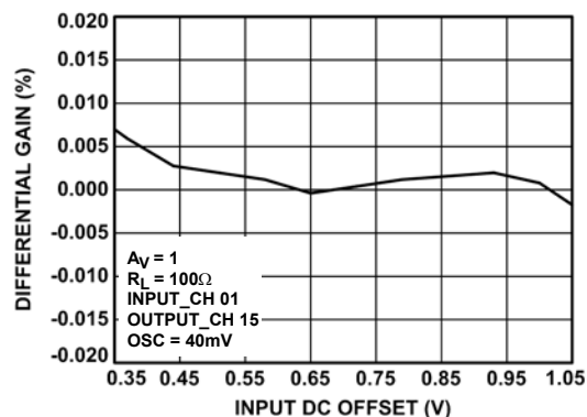
FIGURE 41. DIFFERENTIAL GAIN, A_V = 1
