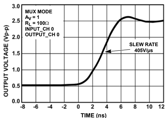
FIGURE 21. RISING SLEW RATE - A_V = 1
