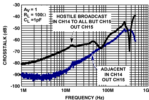
FIGURE 11. CROSSTALK - A_V = 1
