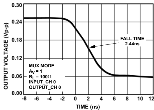
FIGURE 18. FALL TIME - A_V = 1
