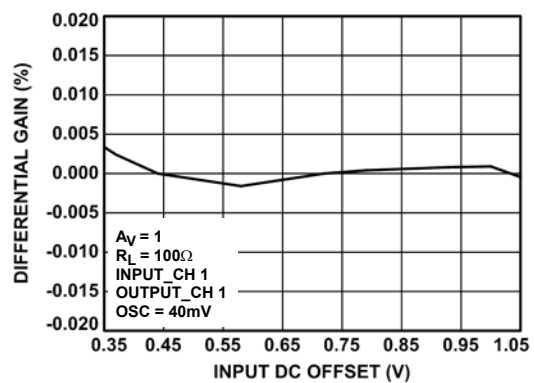
FIGURE 33. DIFFERENTIAL GAIN, A_V = 1
