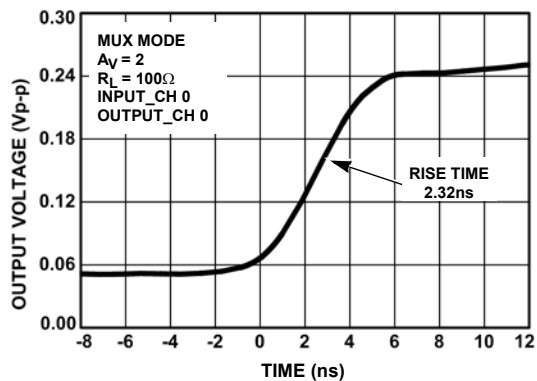
FIGURE 19. RISE TIME - A_V = 2
