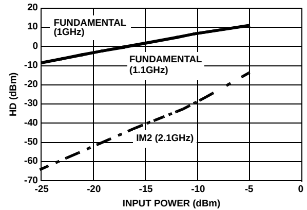
FIGURE 8. IM2 vs INPUT POWER
