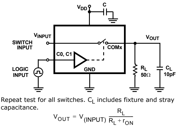
FIGURE 1B. ADDRESS t_{TRANS} TEST CIRCUIT
