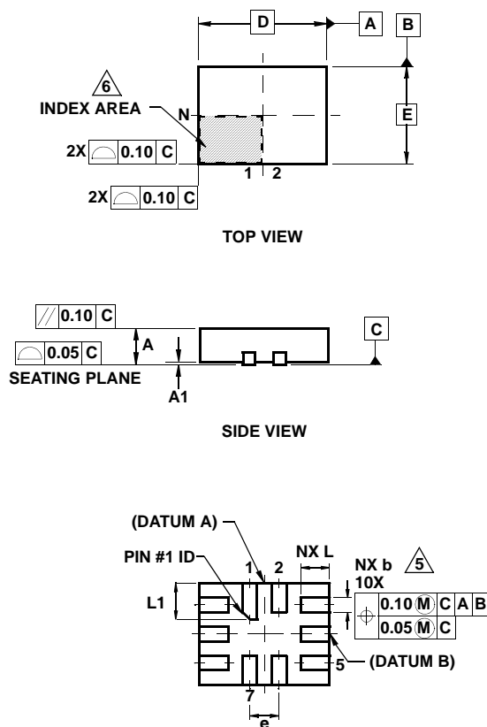
BOTTOM VIEW
