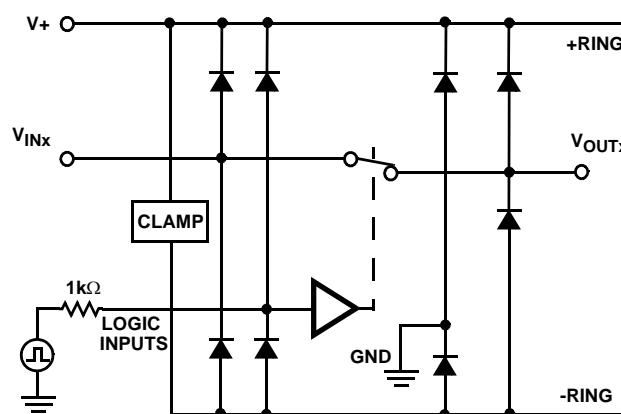
FIGURE 8. OVERVOLTAGE PROTECTION
