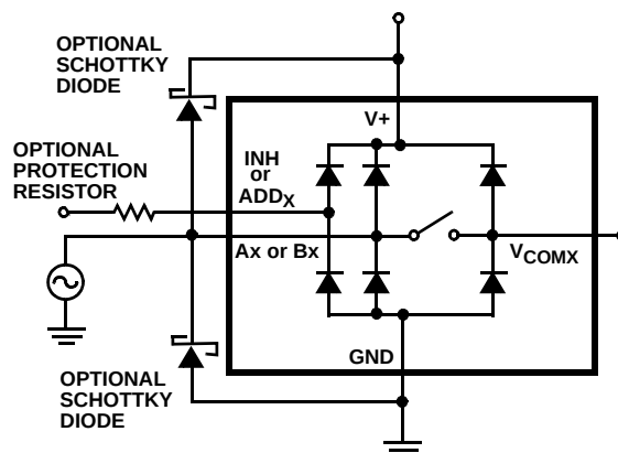
FIGURE 7. OVERVOLTAGE PROTECTION
