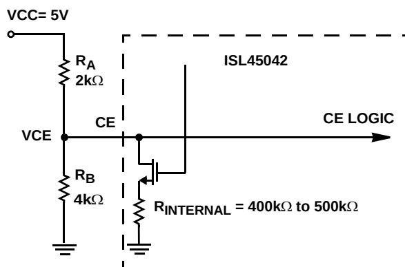
FIGURE 5. APPLICATION GENERATING VDD AND VCE VOLTAGES
