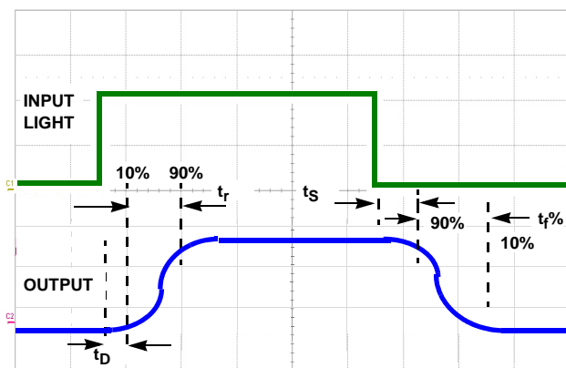
FIGURE 2. TIMING DIAGRAM
