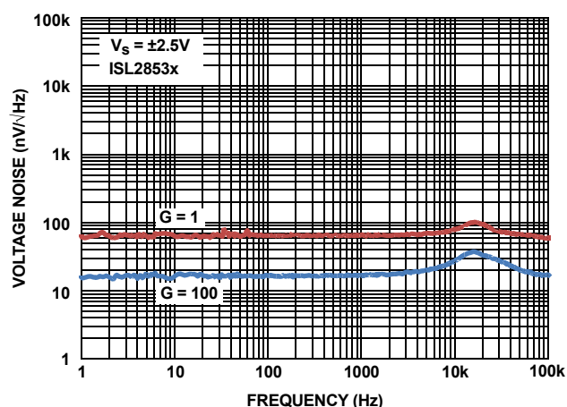
FIGURE 31. PGIA VOLTAGE NOISE SPECTRAL DENSITY vs FREQUENCY, 1Hz TO 100kHz
