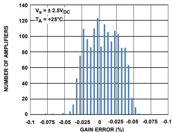
FIGURE 9. PGIA GAIN ERROR DISTRIBUTION, G = 1 \text{ TO } 1,000
