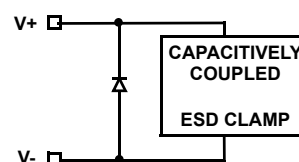
CIRCUIT 3
