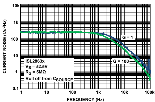
FIGURE 34. PGIA CURRENT NOISE SPECTRAL DENSITY 1Hz TO 100kHz, ISL2863x
