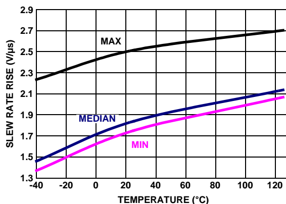
FIGURE 35. SLEW RATE RISE vs TEMPERATURE, V_{OUT} = \pm 1.5V , V_{P-P} = 2.5V , V_+ = 5V , V_- = 0V , V_{CM} = 2.5V , R_L = 100k
