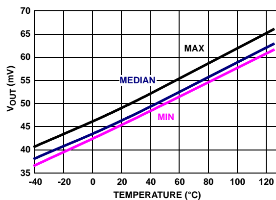
FIGURE 32. V_{OUT} LOW vs TEMPERATURE, V_+ = 5V , V_- = 0V , V_{CM} = 2.5V , R_L = 1k
