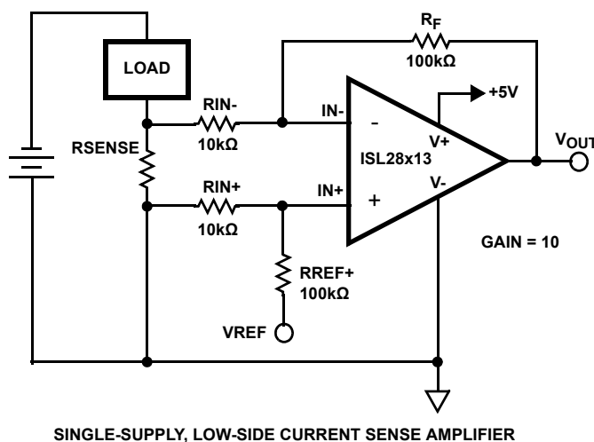
FIGURE 1. TYPICAL APPLICATION
