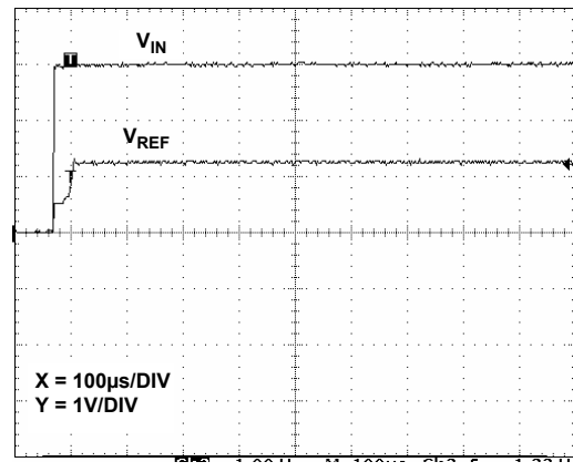
FIGURE 11. TURN-ON TIME
