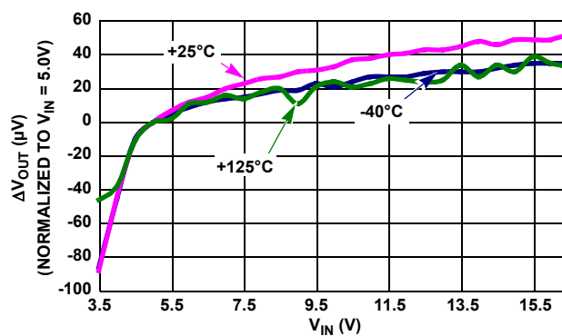
FIGURE 19. LINE REGULATION OVER-TEMPERATURE
