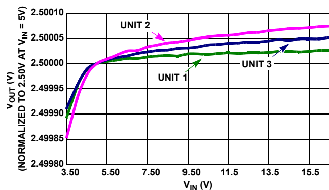
FIGURE 18. LINE REGULATION
