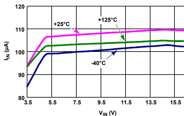
FIGURE 17. I_{IN} vs V_{IN} , 3 TEMPERATURES
