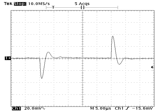
FIGURE 23. LINE TRANSIENT RESPONSE, NO CAPACITIVE LOAD
