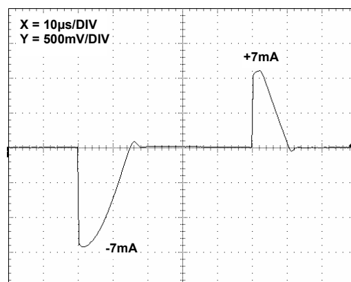
FIGURE 15. LOAD TRANSIENT RESPONSE
