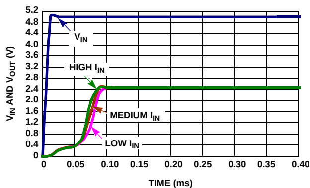
FIGURE 25. TURN-ON TIME
