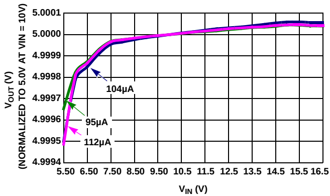
FIGURE 46. LINE REGULATION
