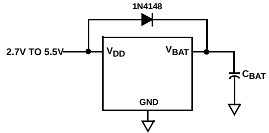
FIGURE 21. SUPERCAPACITOR CHARGING CIRCUIT
