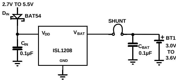
FIGURE 20. POWER GLITCH PROTECTION CIRCUIT
