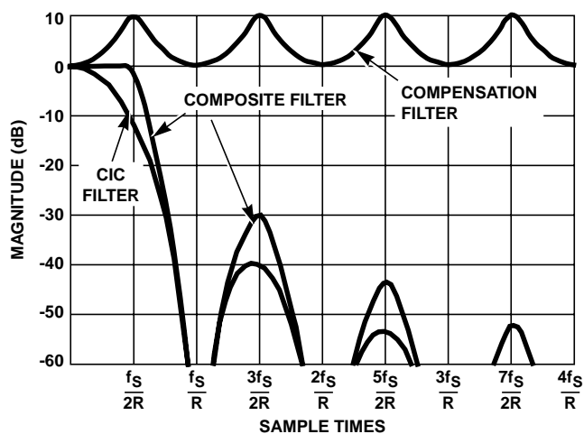
FIGURE 7. THIRD ORDER CIC FREQUENCY RESPONSE
