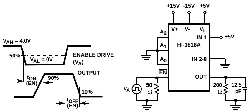
FIGURE 1B. TEST CIRCUIT
