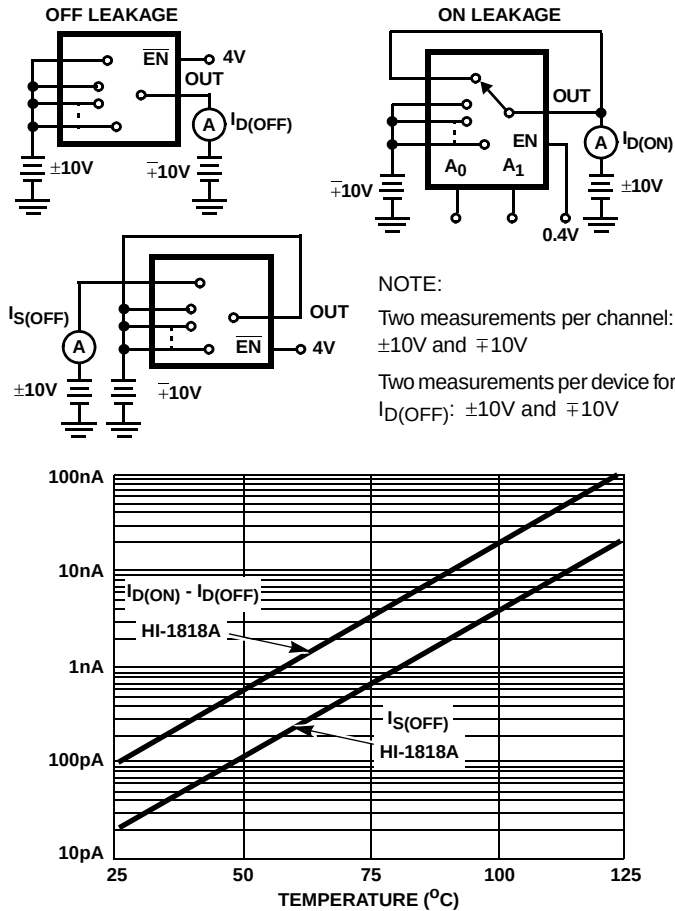
FIGURE 5. LEAKAGE CURRENTS vs TEMPERATURE
