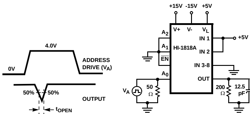
FIGURE 2B. TEST CIRCUIT
