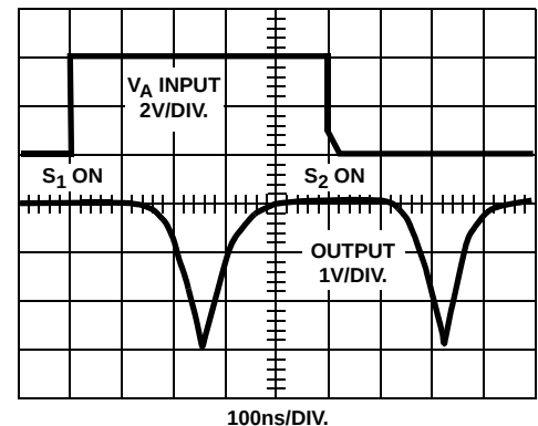
FIGURE 2C. WAVEFORMS
