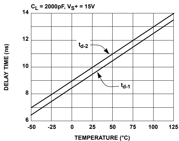
FIGURE 8. PROPAGATION DELAY vs TEMPERATURE
