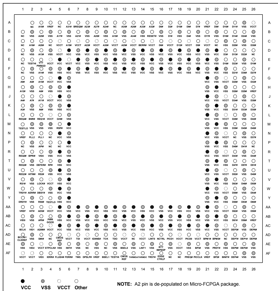
Figure 29. Pin/Ball Map - Top View
