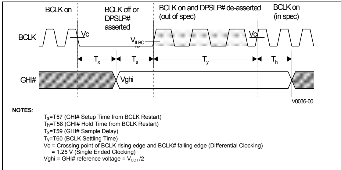
Figure 19. Enhanced Intel SpeedStep Technology/Deep Sleep Timing
