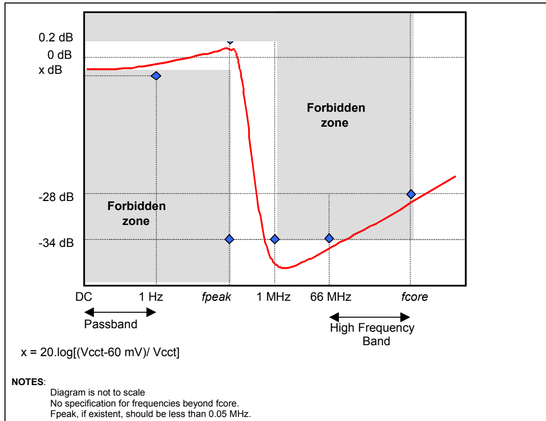
Figure 30. PLL Filter Specifications
