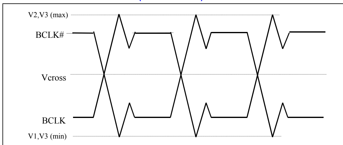
Figure 7. Differential BCLK/BCLK# Waveform (Common Mode)
