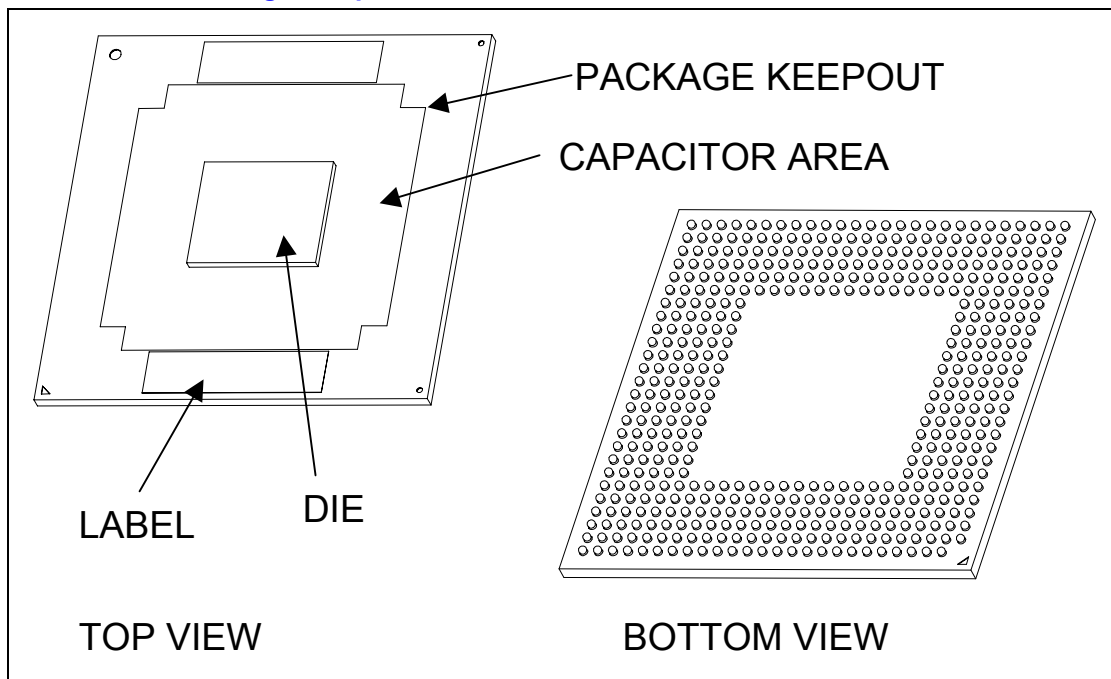
Figure 26. Micro-FCBGA Package – Top and Bottom Isometric Views
