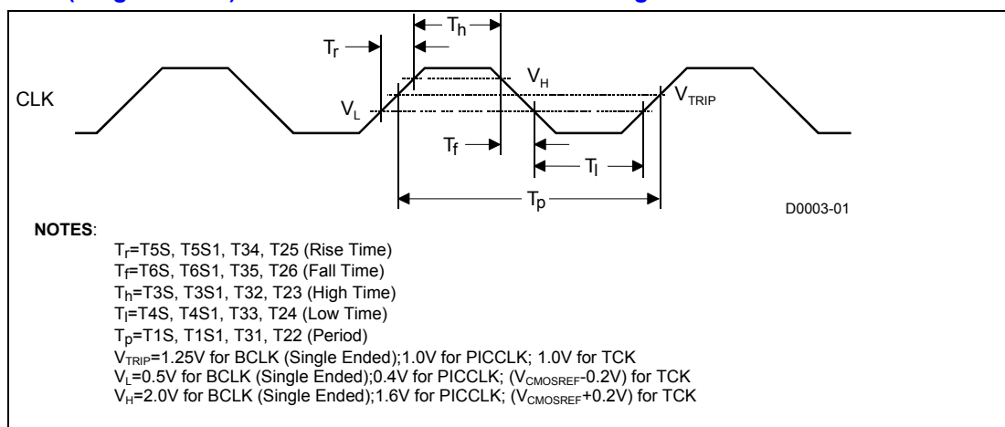
Figure 6. BCLK (Single Ended)/PICCLK/TCK Generic Clock Timing Waveform
