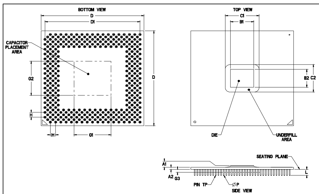
Figure 23. Package Dimensions (FC-PGA Package)
