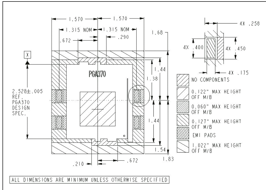
Figure 41. Clip Keepout Requirements for the 370-Pin (Top View)
