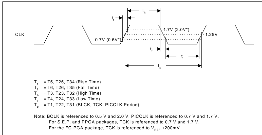
Figure 4. System Bus Valid Delay Timings
