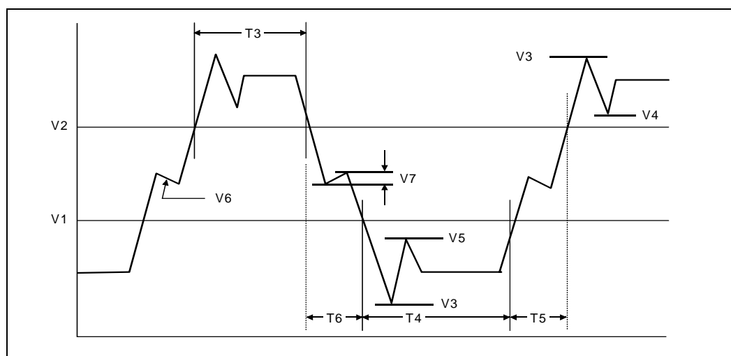
Figure 12. BCLK, TCK, PICCLK Generic Clock Waveform at the Processor Edge Fingers
