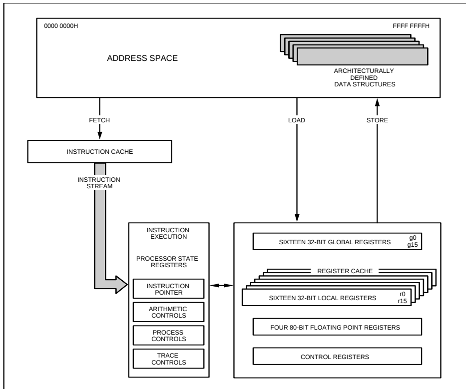
Figure 2. 80960KB Programming Environment
