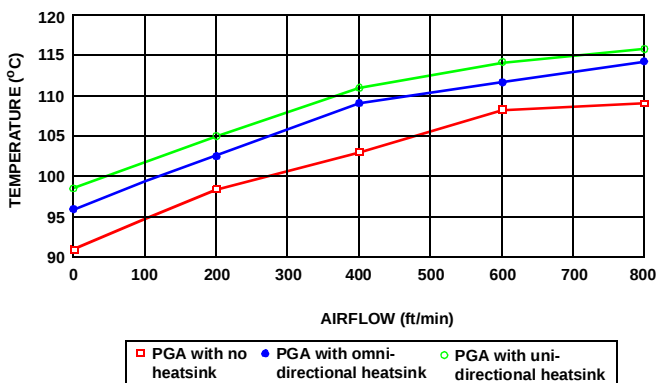
Figure 26. Maximum Allowable Ambient Temperature for the Extended Temperature TA-80960KB at 20 MHz in PGA Package
