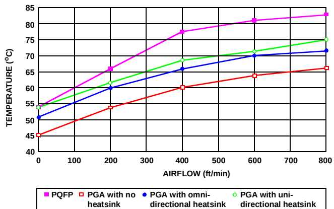
Figure 25. 25 MHz Maximum Allowable Ambient Temperature
