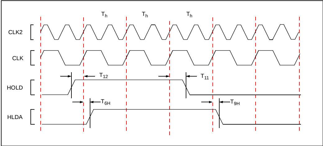
Figure 22. HOLD Timing
