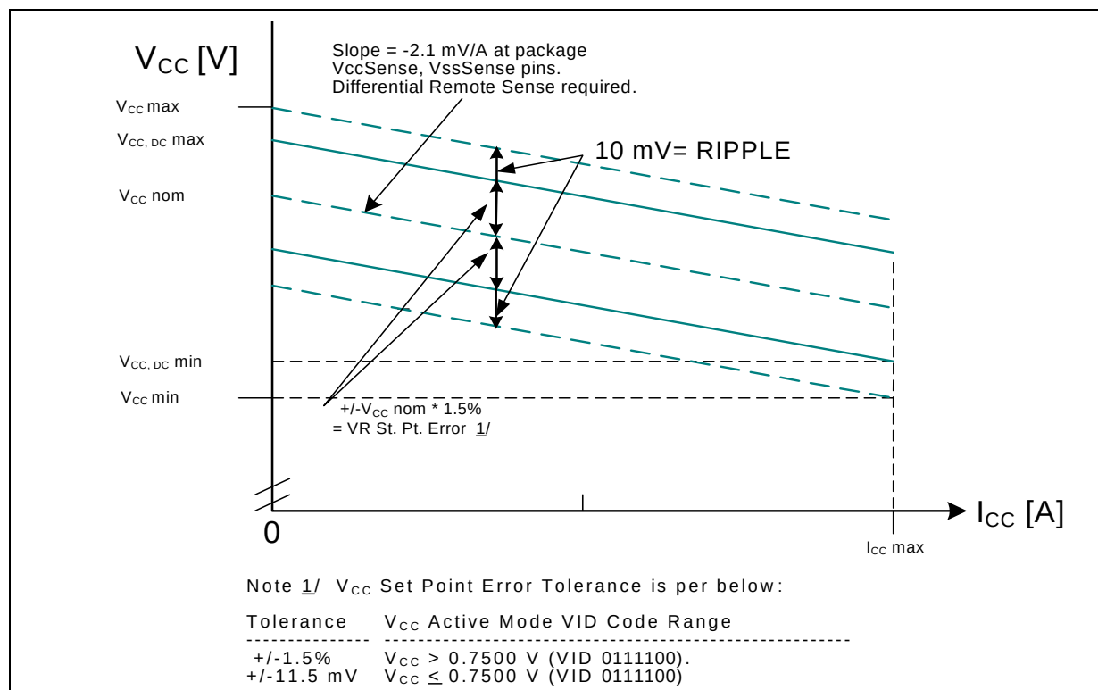
Figure 3. Active V_{CC} and I_{CC} Loadline Standard Voltage
