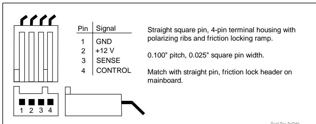
Figure 30. Boxed Processor TMA Power Cable Connector Description
