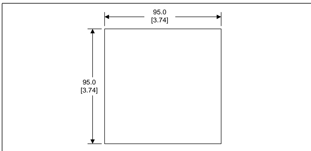
Figure 19. Space Requirements for the Boxed Processor (Top View)
