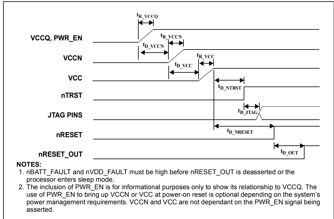
Figure 3. Power-On Reset Timing
