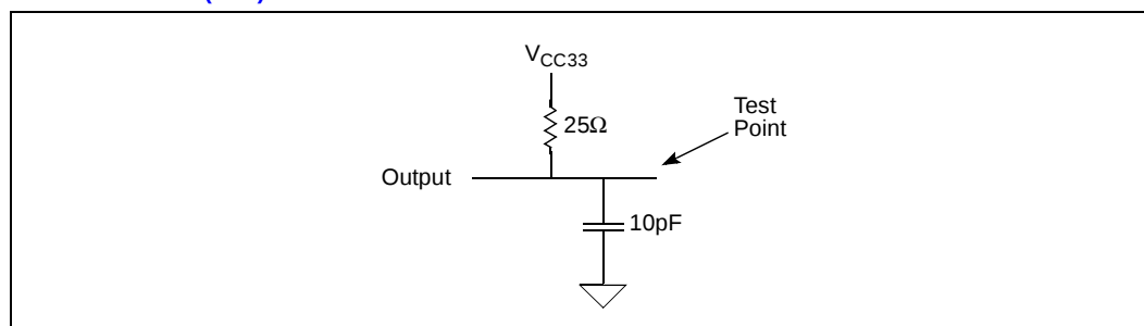
Figure 16. PCI/PCI-X T_{OV(max)} Falling Edge AC Test Load
