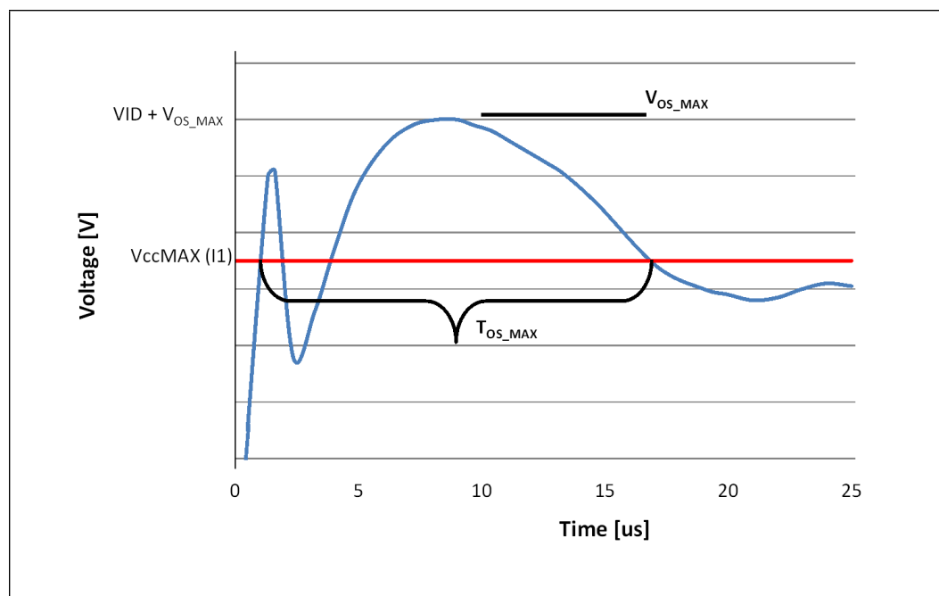
Figure 7-3. V_{CC} Overshoot Example Waveform
