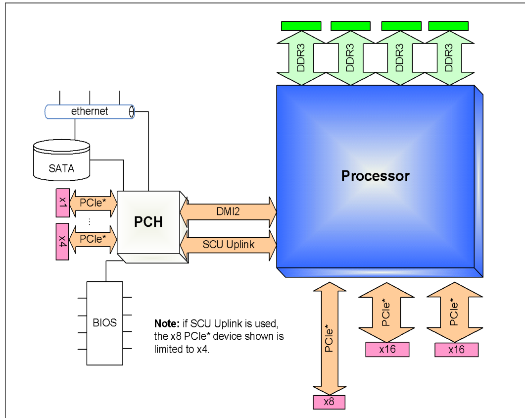
Figure 1-1. Processor Platform Block Diagram Example
