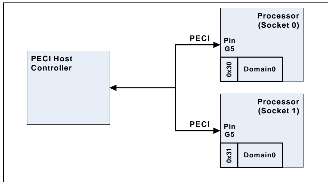
Figure 6-8. Dual-Core Intel® Xeon® Processor 5200 Series PECI Topology
