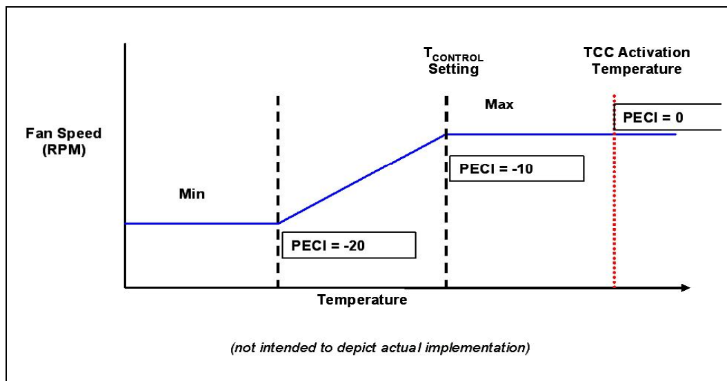
Figure 16. Conceptual Fan Control Diagram on PEGI-Based Platforms
