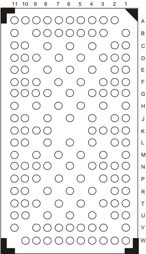
BOTTOM VIEW
