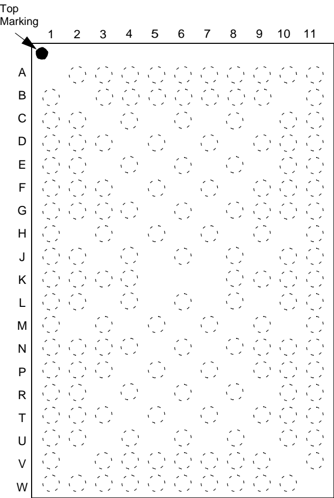
TOP VIEW
