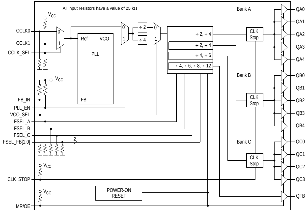
Figure 1. MPC97H74 Logic Diagram
