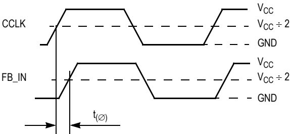
Figure 13. Propagation Delay ( t_{PD} , static phase offset) Test Reference
