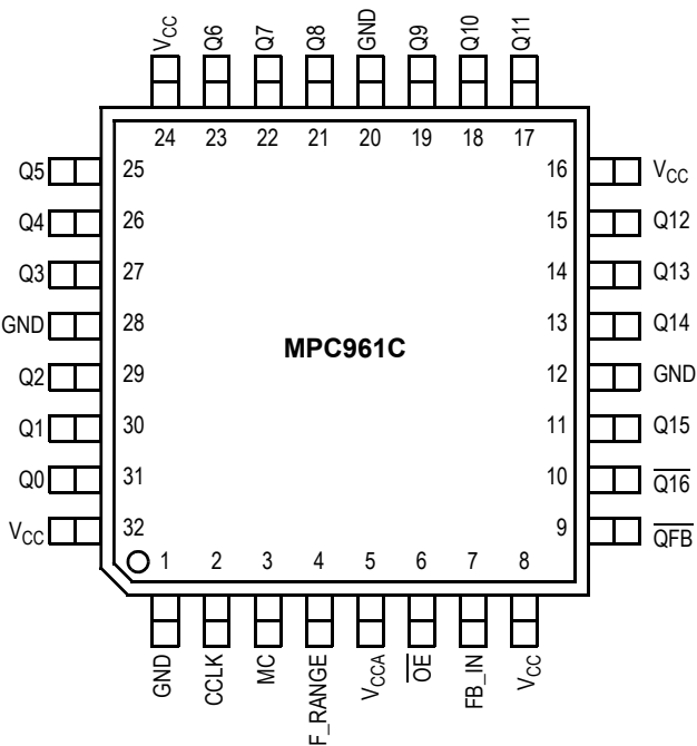
Figure 2. 32-Lead Pinout (Top View)
