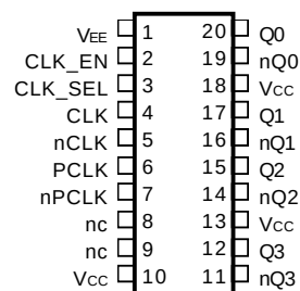
ICS8533-01 20-Lead TSSOP 6.5mm x 4.4mm x 0.92mm Package Body G Package Top View
