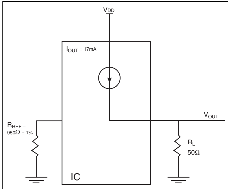
Figure 5. HCSSL Driver Circuit and Termination
