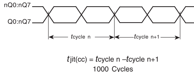
CYCLE-TO-CYCLE JITTER
