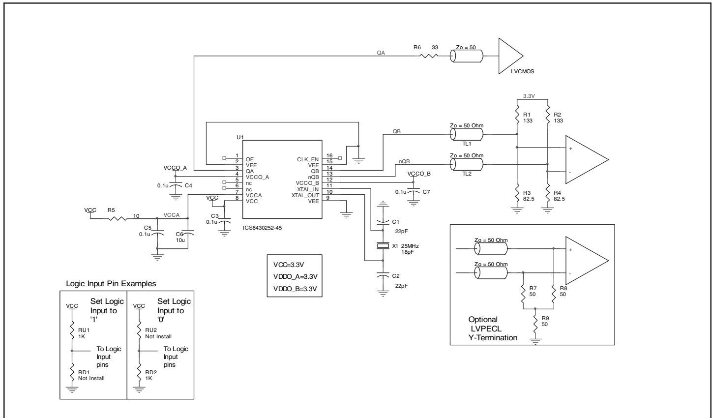
FIGURE 5. ICS8430252-45 SCHEMATIC EXAMPLE
