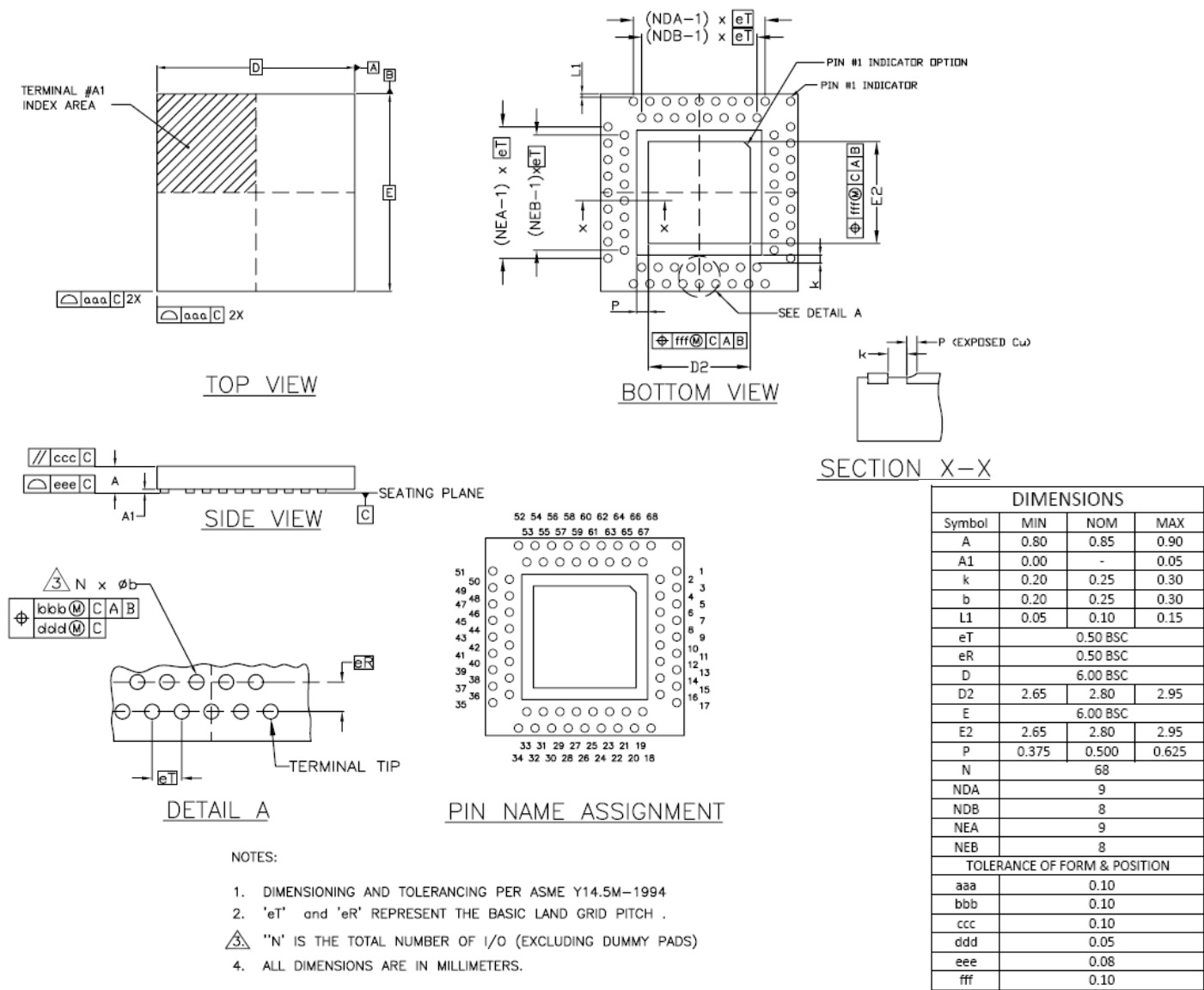
Figure 36. Package Outline
