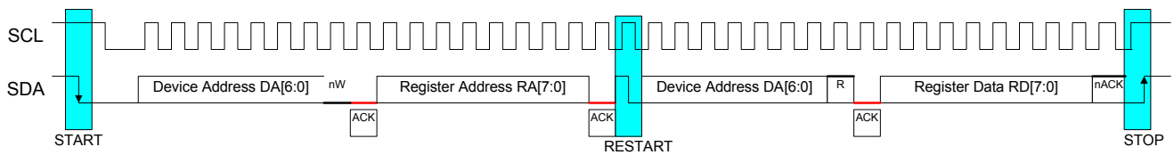
Figure 32. Read Cycle
