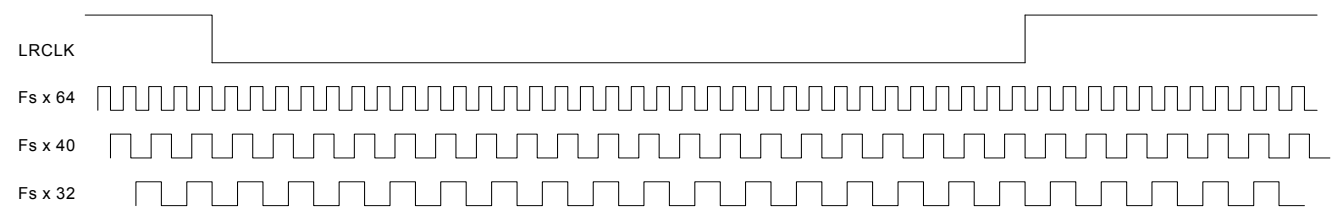
Figure 29. Bit Clock mode
