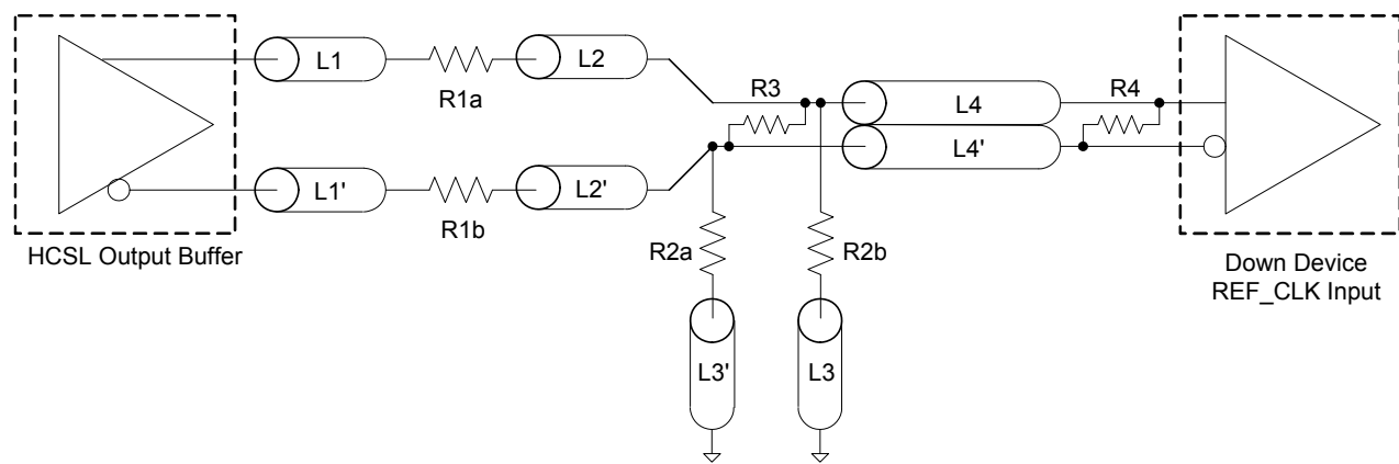
Termination for Cable AC Coupled Application (figure 4)
