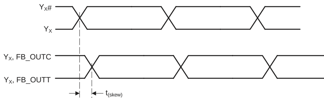
Figure 5. Output Skew
