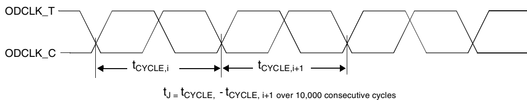
Figure 5. Cycle-to-cycle Jitter
