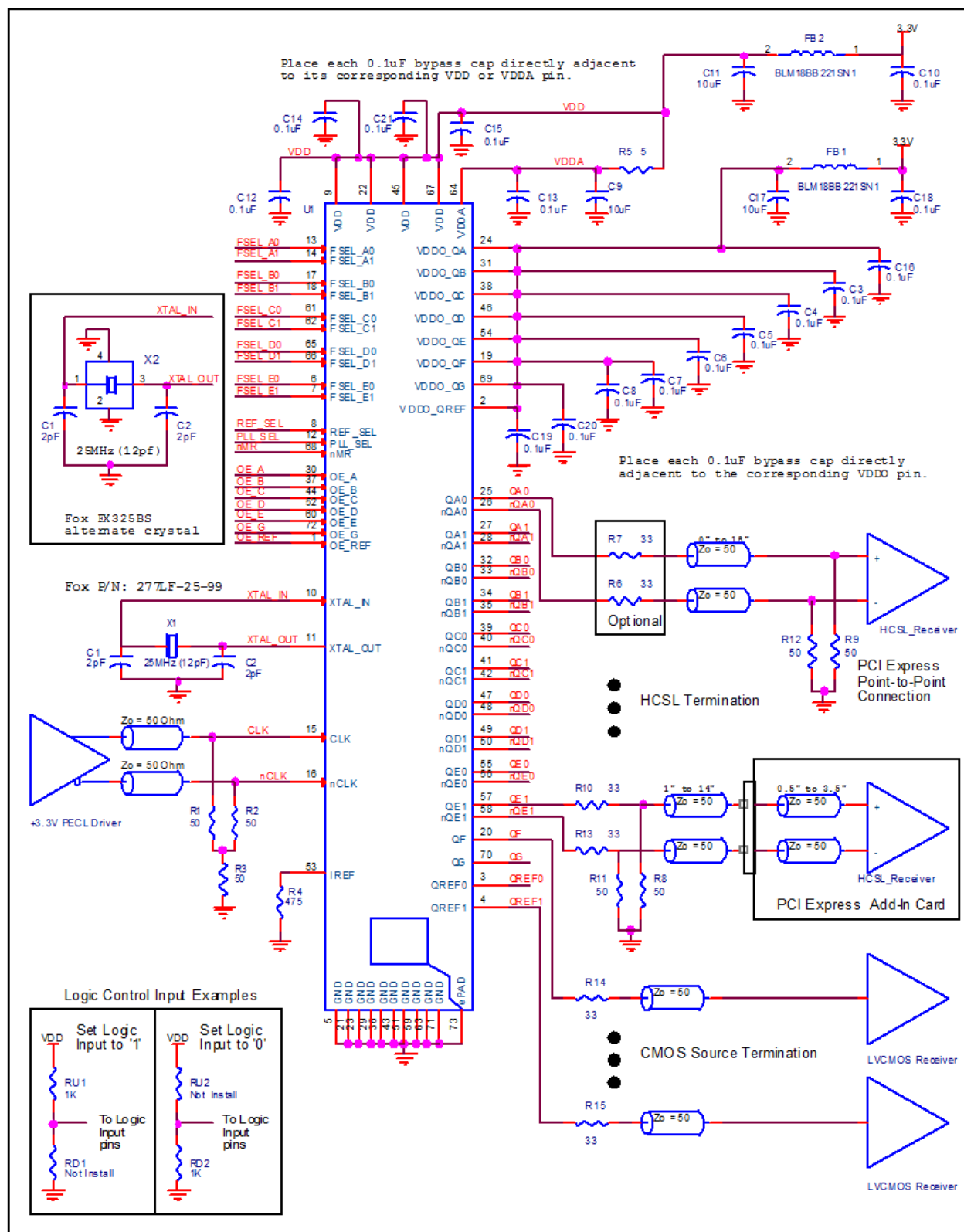
Figure 6. IDT8V41N012I Schematic Example
