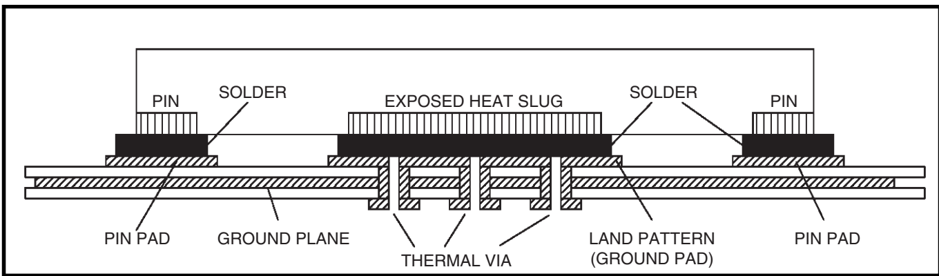
Figure 4. Assembly for Exposed Pad Thermal Release Path - Side View (drawing not to scale)
