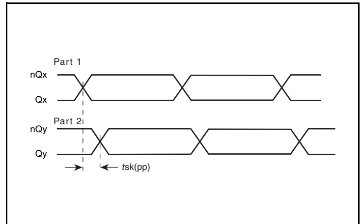
Part-to-Part Skew
