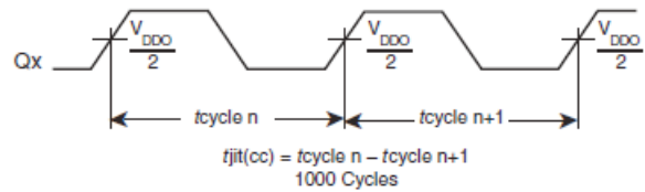
CYCLE-TO-CYCLE JITTER
